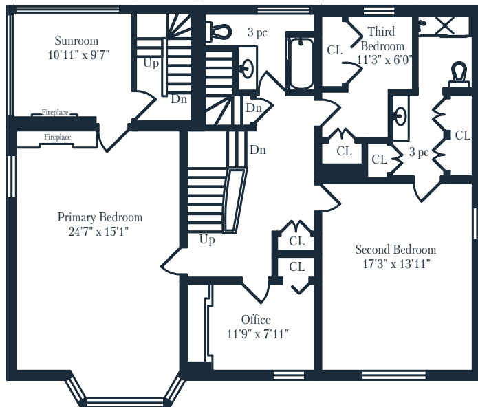
Second Floor 1526 Square Feet
