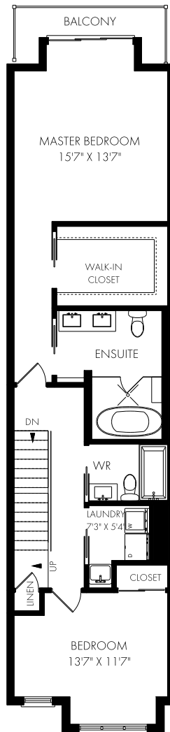
CEILING HEIGHT 9'0" SECOND FLOOR - 875 SQUARE FEET
