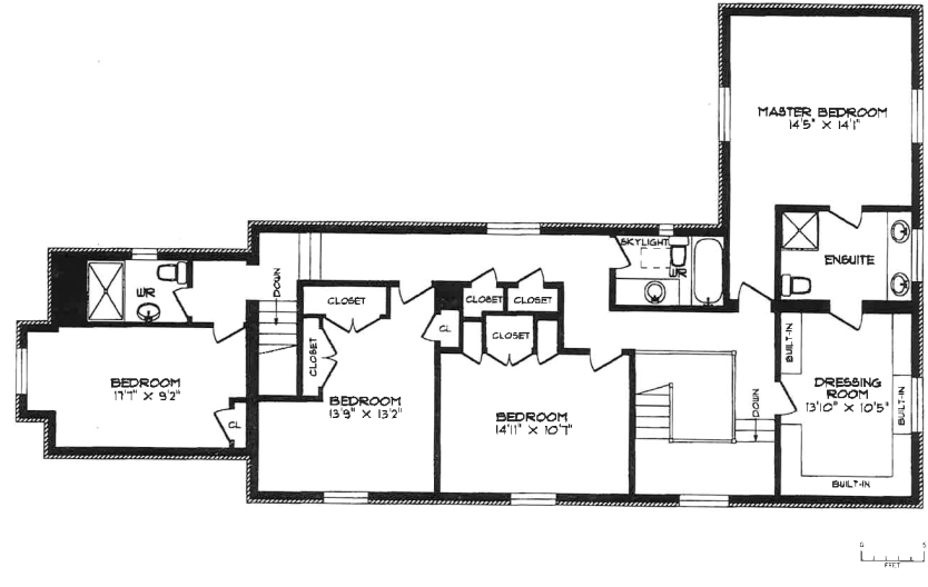
SECOND FLOOR 1676 SQUARE FEET
