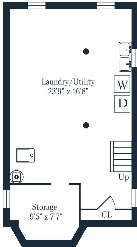
Lower Level 590 Square Feet
